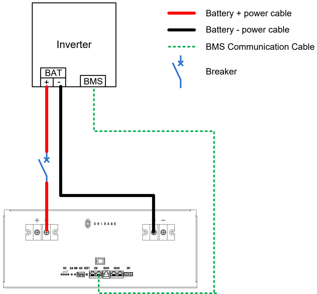
Fig. 4-1 Single CE48100-R PACK + single inverter diagram
