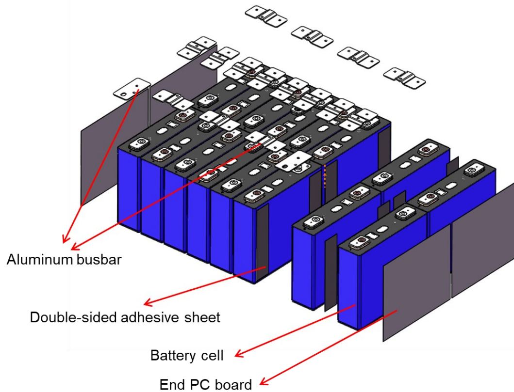
Fig. 3-2 CE48100-R PACK mechanical structure 2
