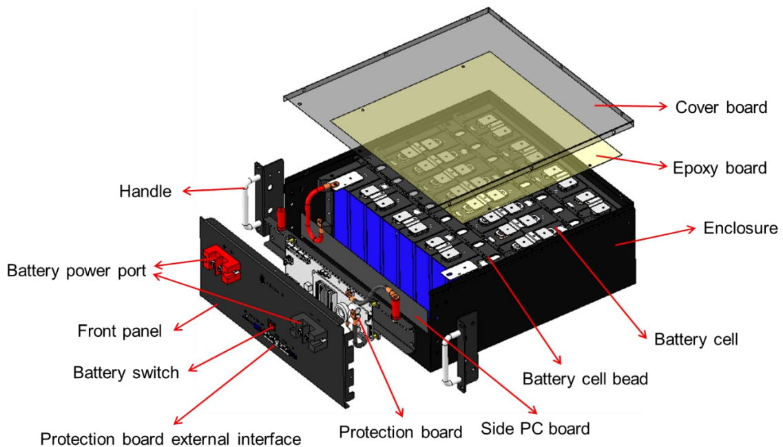
Fig. 3-1 CE48100-R PACK mechanical structure 1
