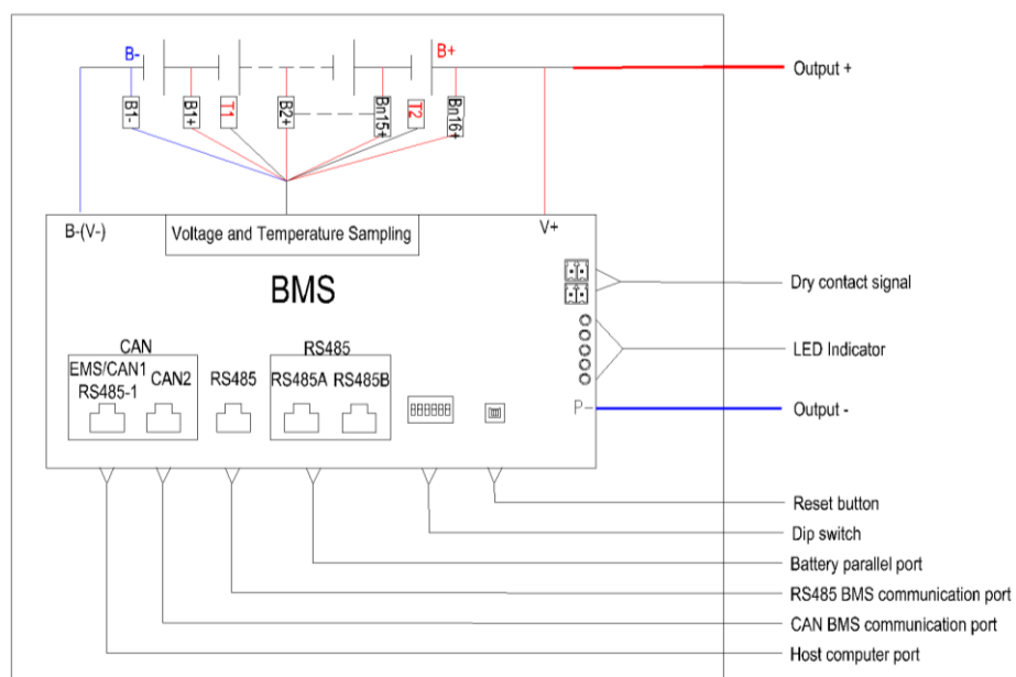
Fig. 3-4 CE48100-R PACK electrical structure
