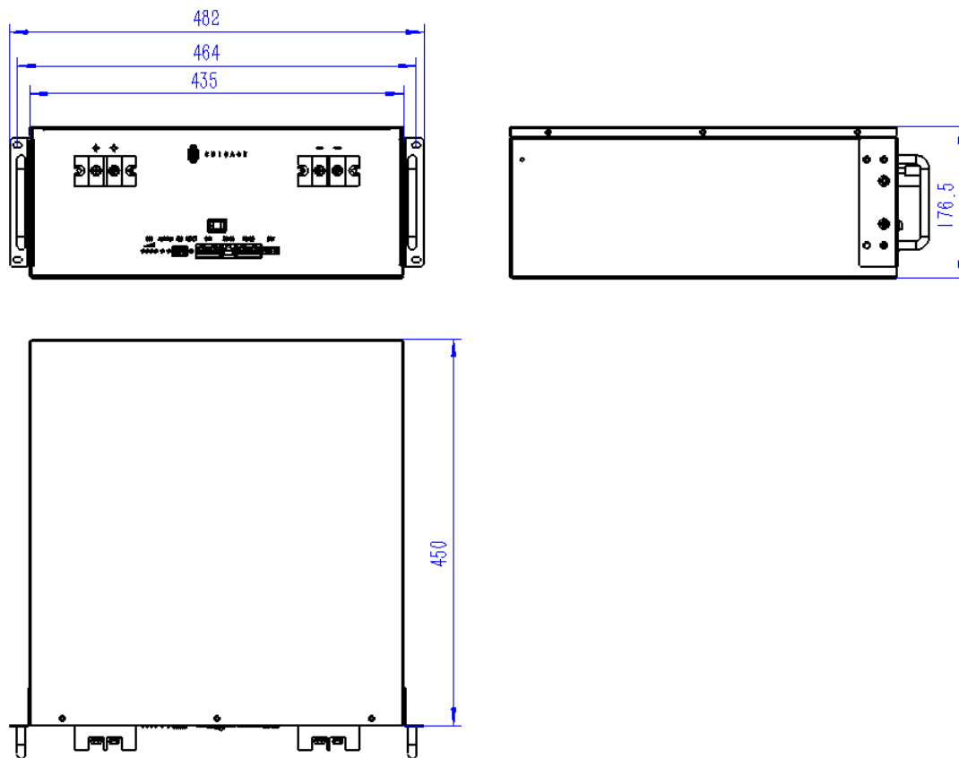
Fig. 3-3 CE48100-R PACK dimension drawing
