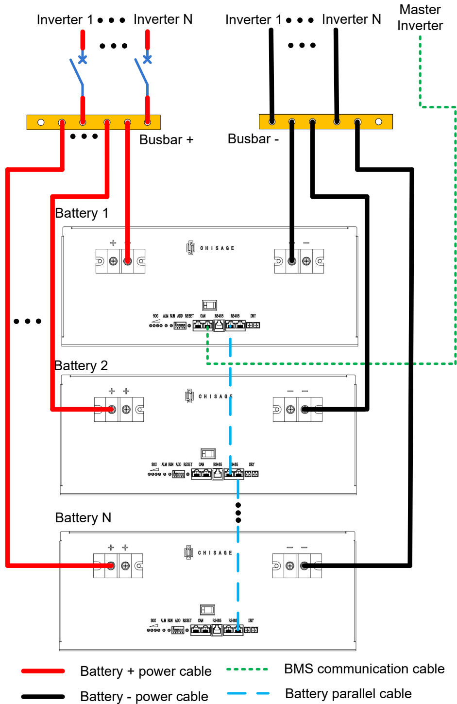
Fig. 4-2 Multi CE48100-R PACK + multi inverter diagram
