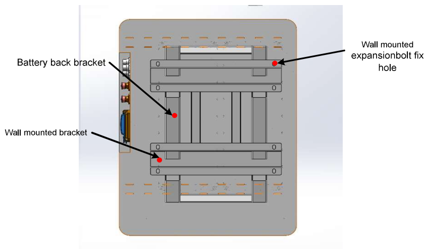
Fig. 3-1 CE48100-W PACK mechanical structure 1
