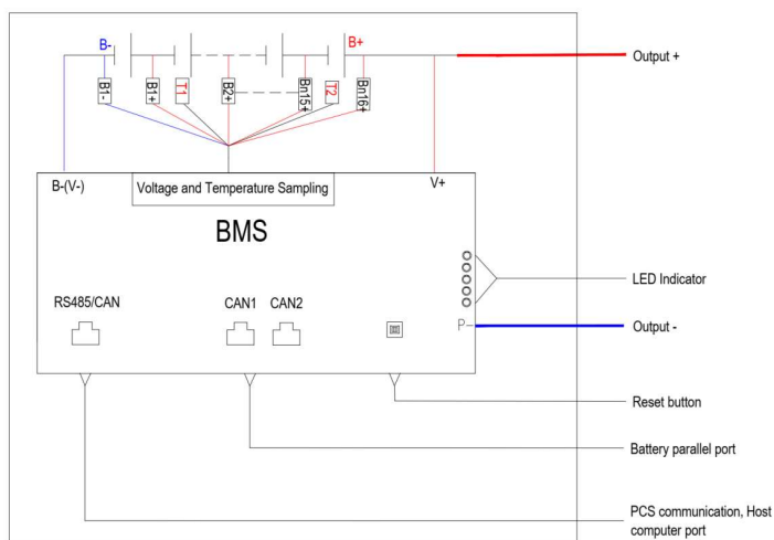
Fig. 3-4 CE48100-W PACK electrical structure
