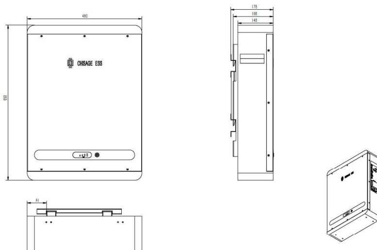
Fig. 3-3 CE48100-W PACK dimension drawing
