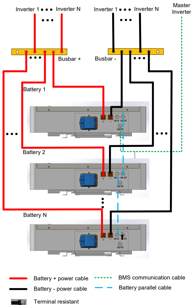
Fig. 4-2 Multi CE48100-W PACK + multi inverter diagram
