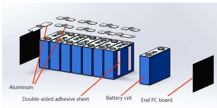
Fig. 3-2 CE48100-W PACK mechanical structure 2
