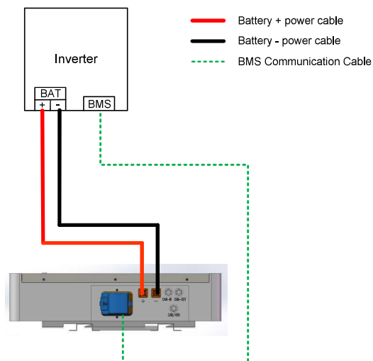
Fig. 4-1 Single CE48100-W PACK + single inverter diagram
